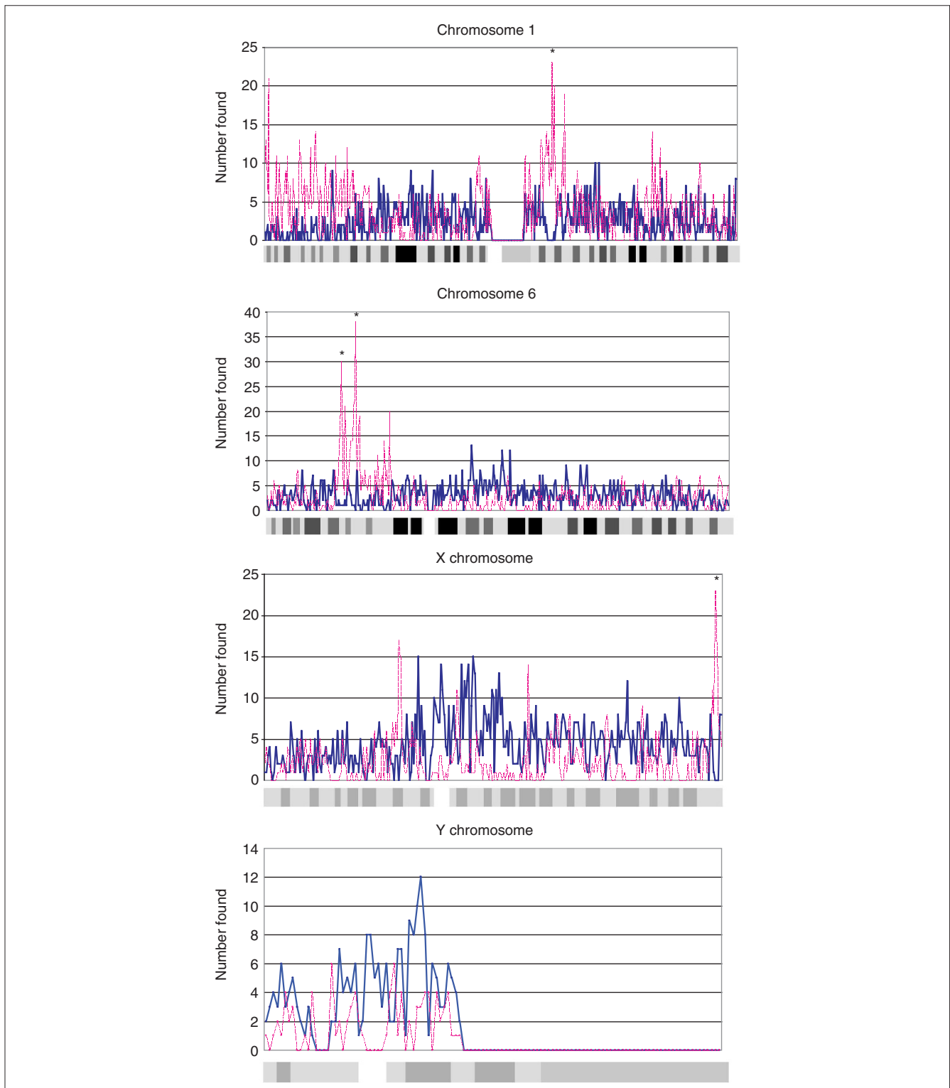
Figure 8 Distribution of LI with TSDs and annotated genes on chromosomes. Along each 500 kb bin along the chromosomes shown, the total number of LI with TSDs (blue line) and the annotated genes (pink line) are indicated. Stars represent loci at which the LI concentration is quite low and gene concentration is high. Among these loci are the histone gene cluster and MHCIII cluster on chromosome 6, a group of genes subject to X inactivation on the X chromosome, and a group of unrelated genes on chromosome 1. The corresponding cytogenetic staining pattern along the length of the chromosomes is shown below the graphs. Centromeric regions are white, and Giemsa-negative bands are indicated by the lightest gray. For the Giemsa-positive bands, the intensity of the grayscale reflects the staining intensity.
