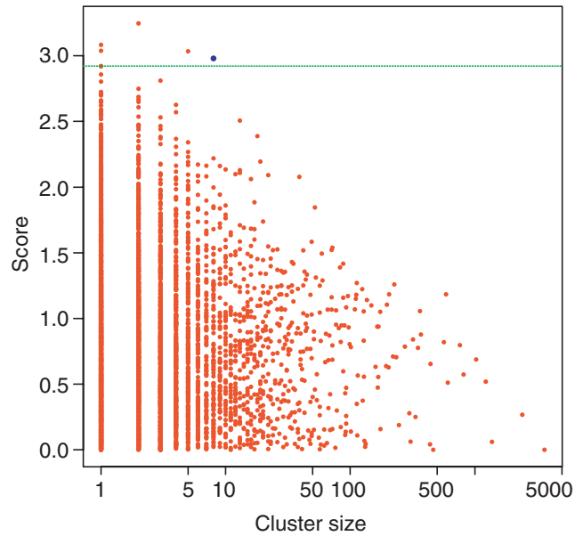
Figure 2 Scores for each cluster, from the first stage of the harvest procedure. The green horizontal line is drawn at (1 - \alpha) times the maximum score, with \alpha = 0.1 . The largest cluster having a score above this line is chosen, indicated by the blue plotting symbol.
